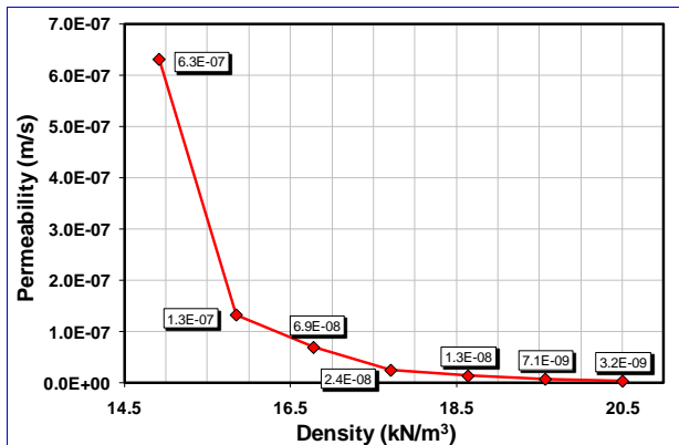
Figure 8. Measured permeability for different densities of the matrix material from Hattian Bala landslide dam
