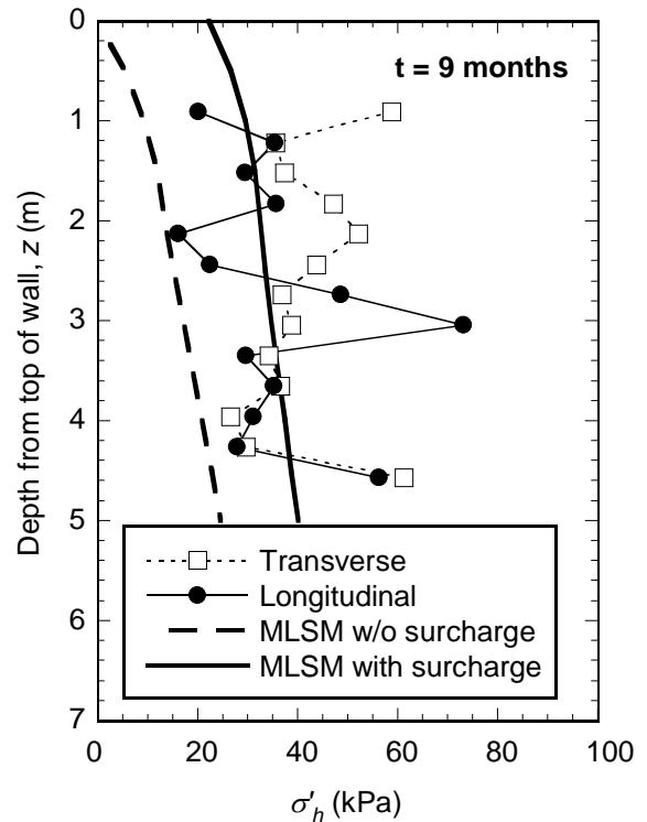
Figure 6 Comparison of measured (DMT) lateral stresses at t = 0, 3, 6, and 9 months after wall construction relative to lateral stresses predicted from modified lateral squeezing model (MLSM) with and without the dike surcharge.
