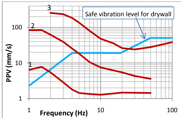
Figure 6. Human sensitivity to vibrations (Wright and Green, 1959) and safe level for drywall as per RI 8507 (Siskind et al, 1980).
