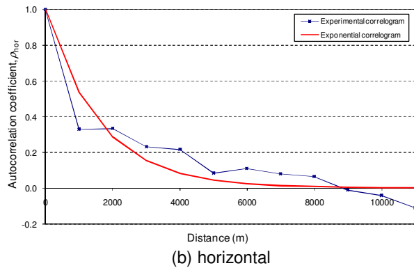
Figure 10. Spatial correlation models for water content
