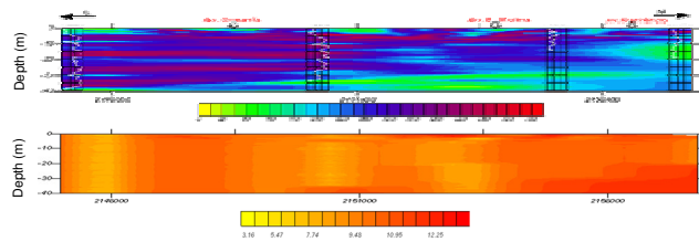
Figure 11. Cross-sections showing variations of estimated water content and associated uncertainty
